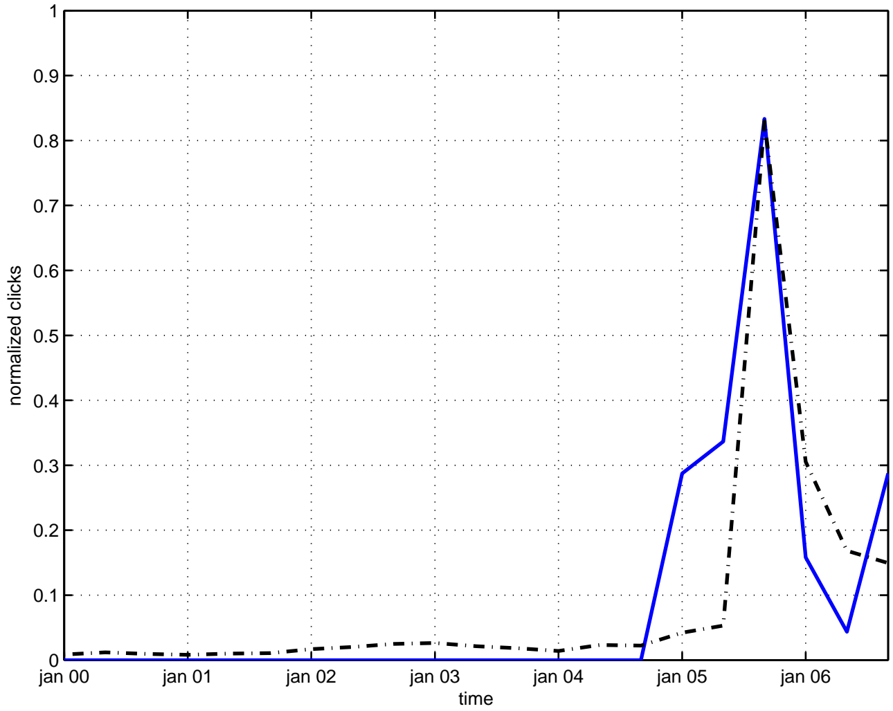
geometrical tachyon
