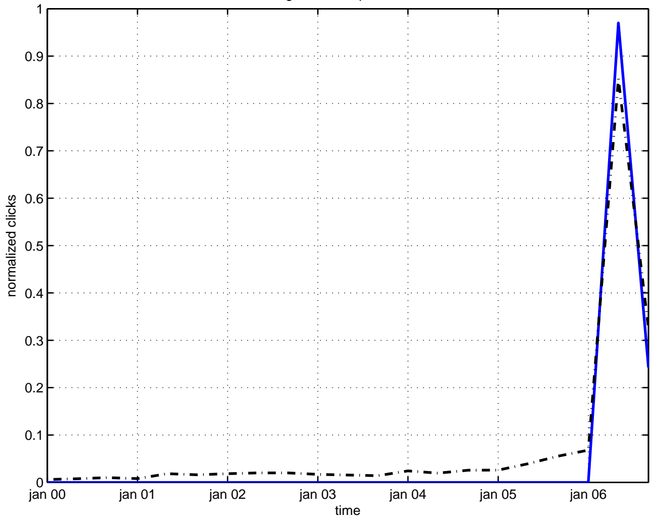
geometrical potential
