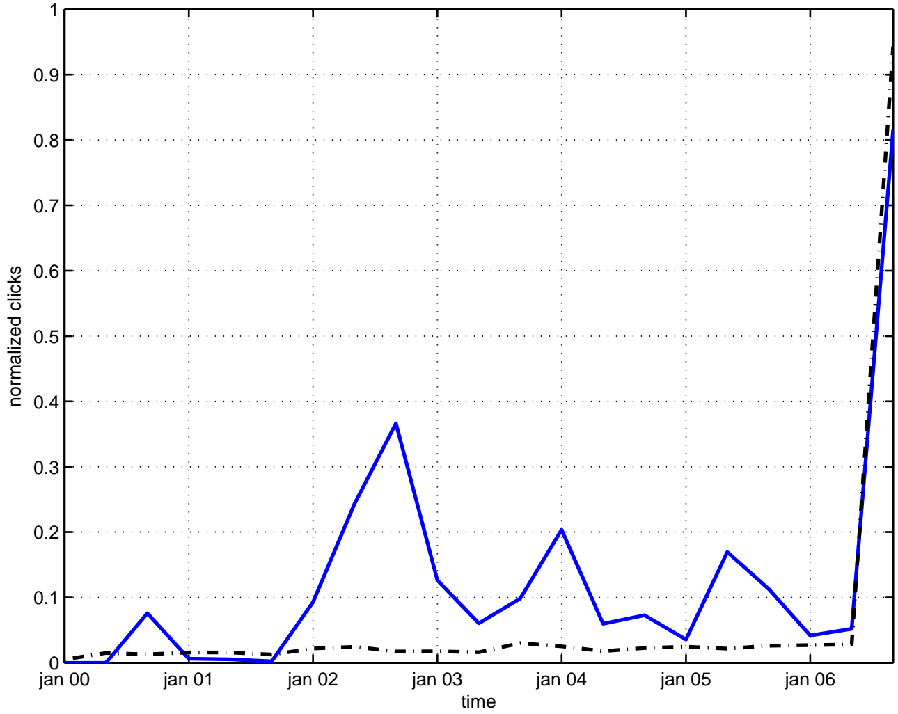
geometrical optics
