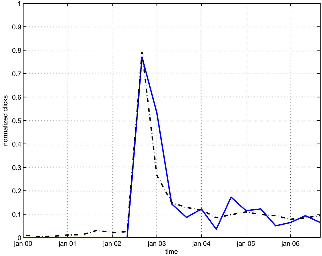
geometrical field theory
