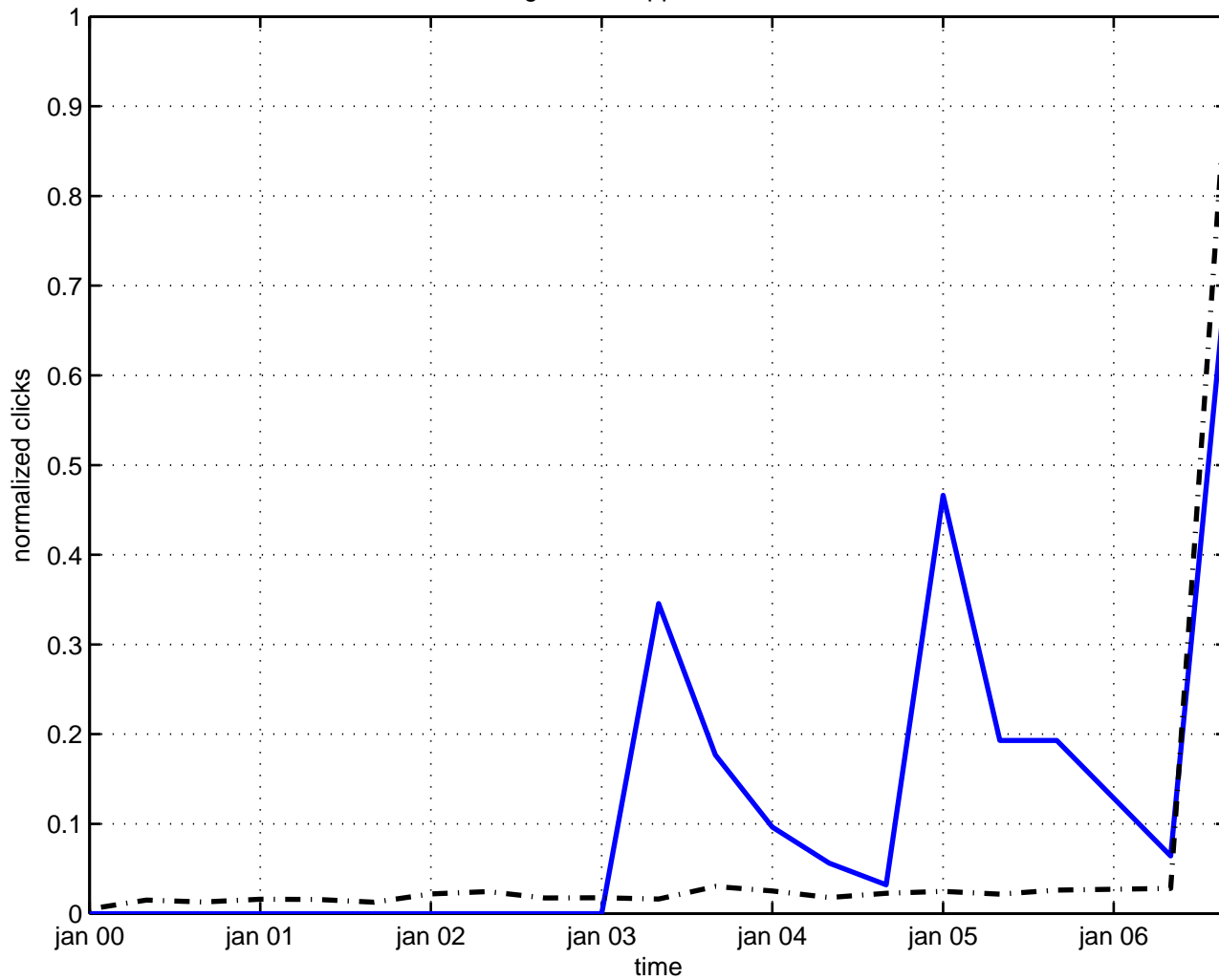
geodesic approximation
