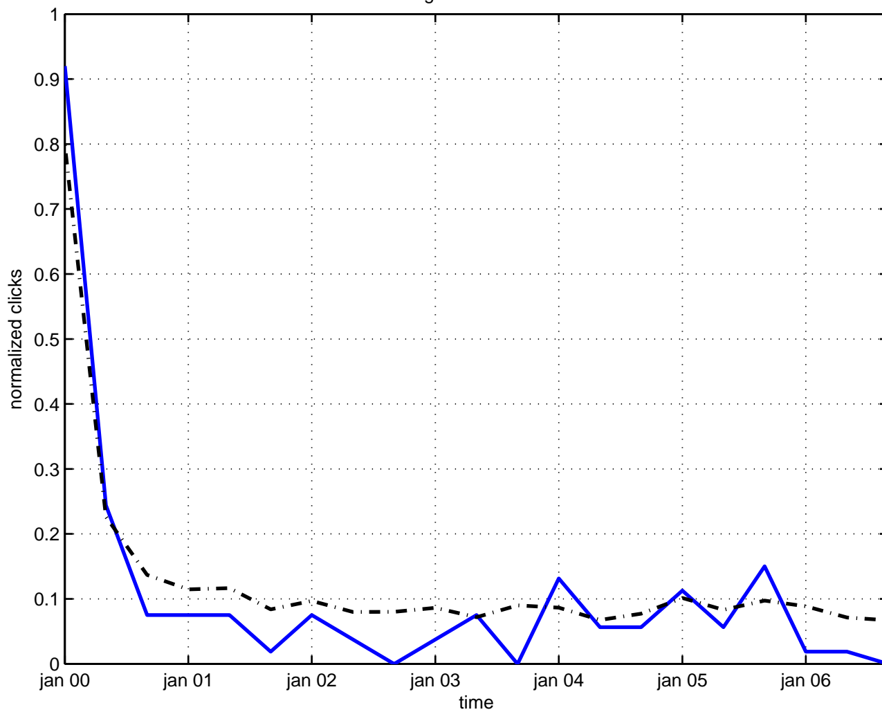
gauss model
