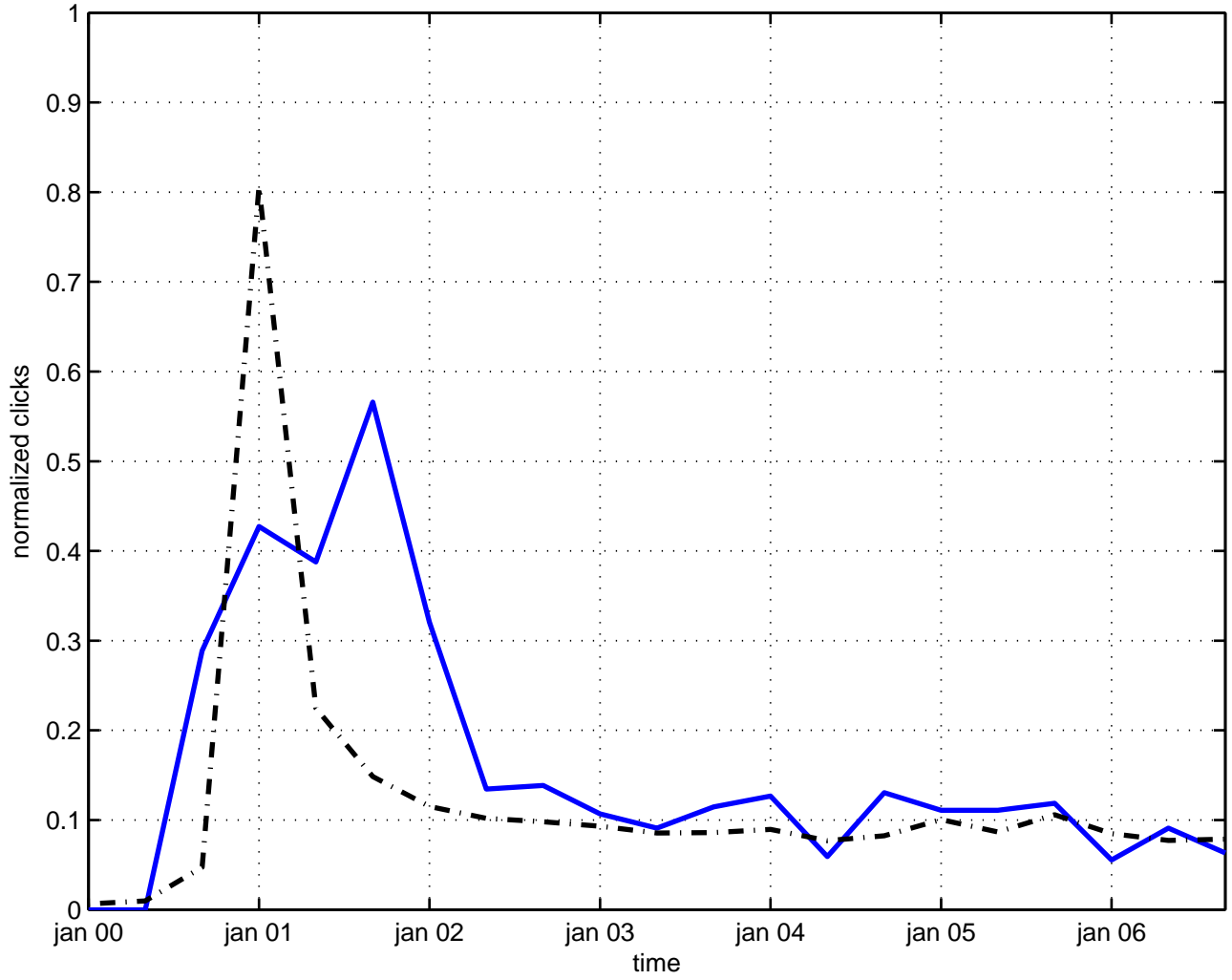
gauss approximation
