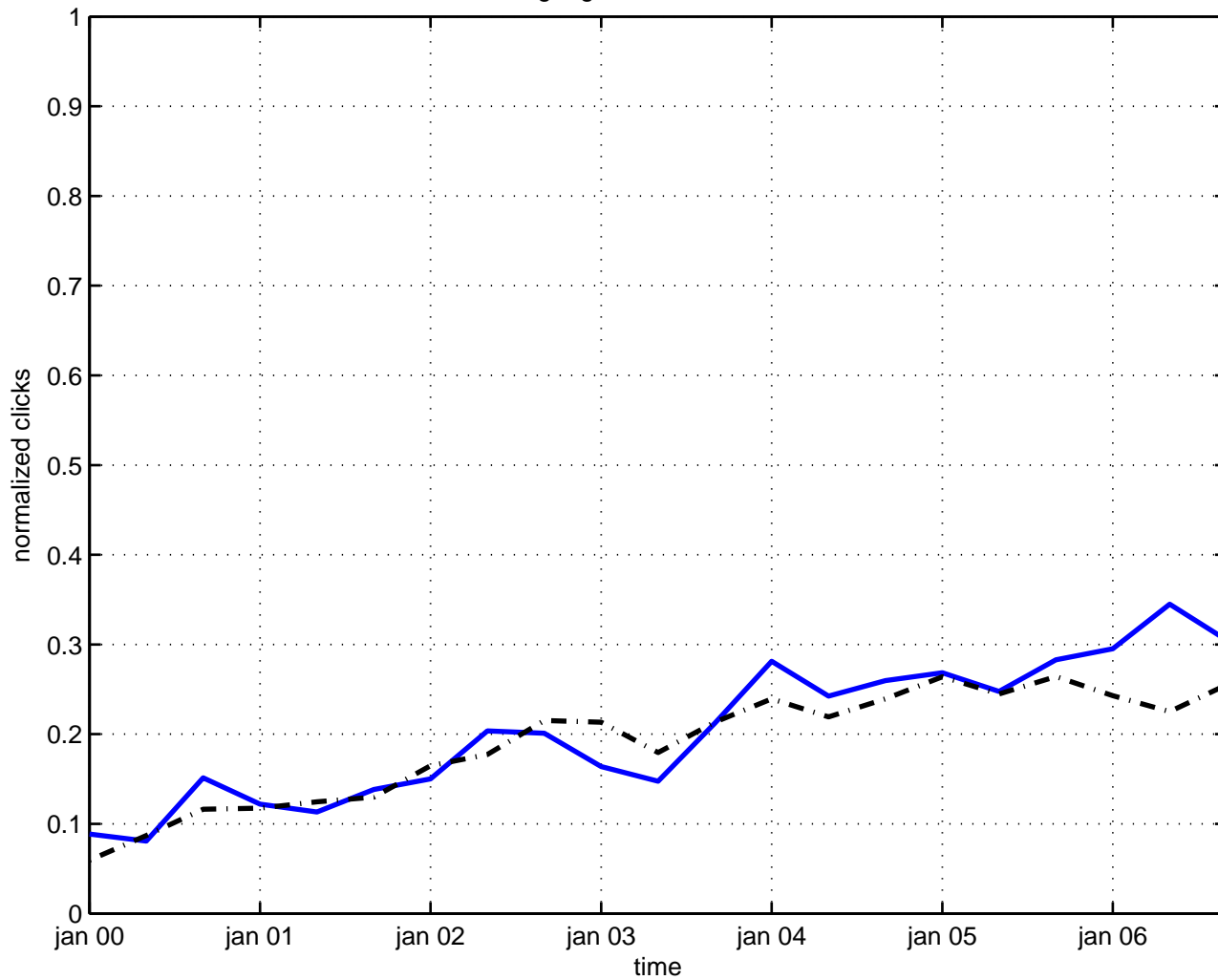
gauge transformation
