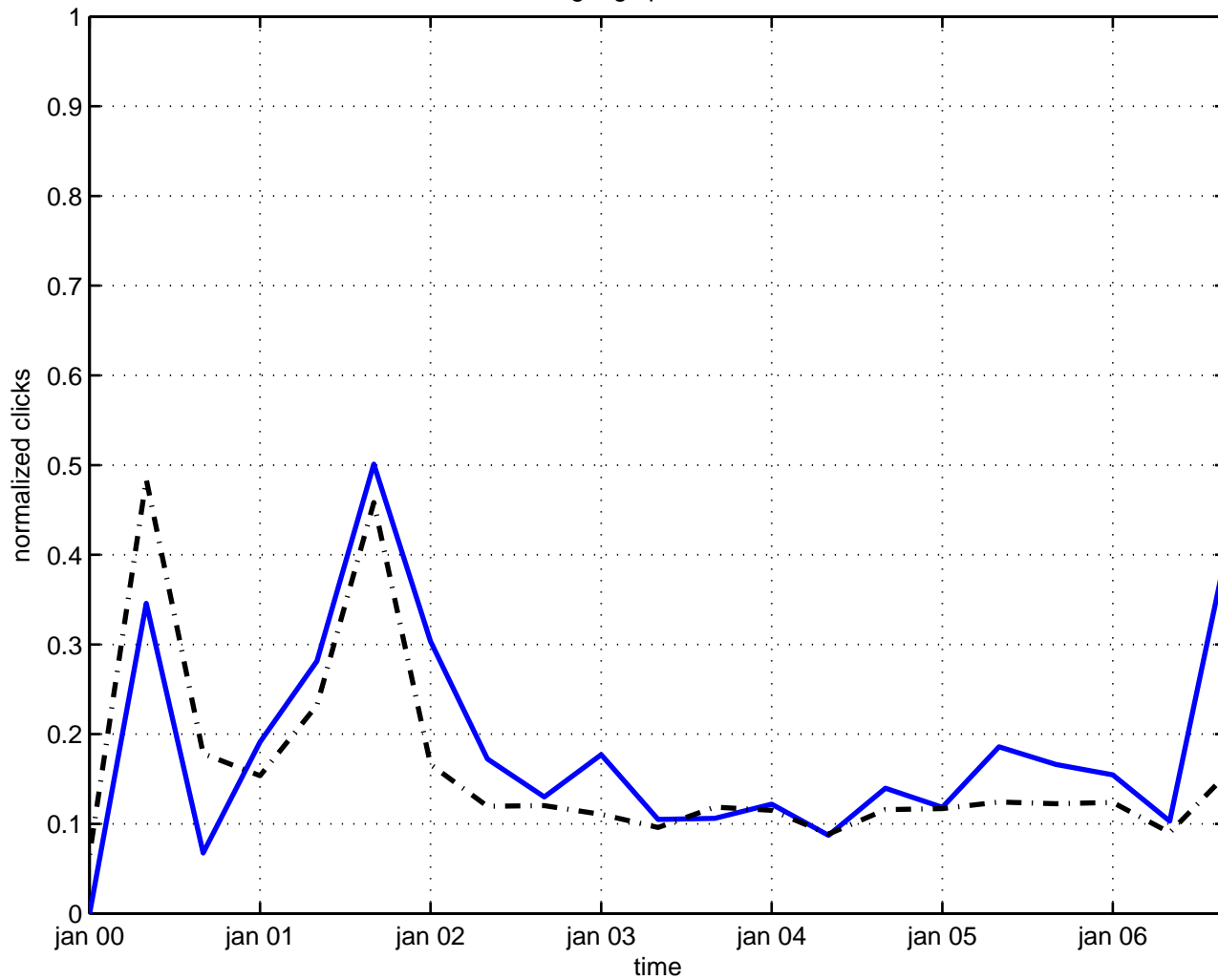
gauge potential
