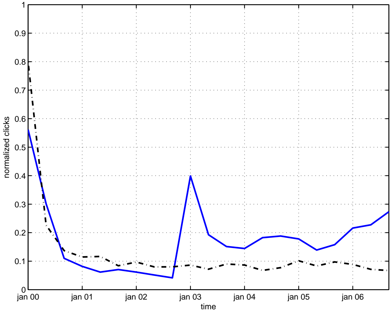
gauge flux
