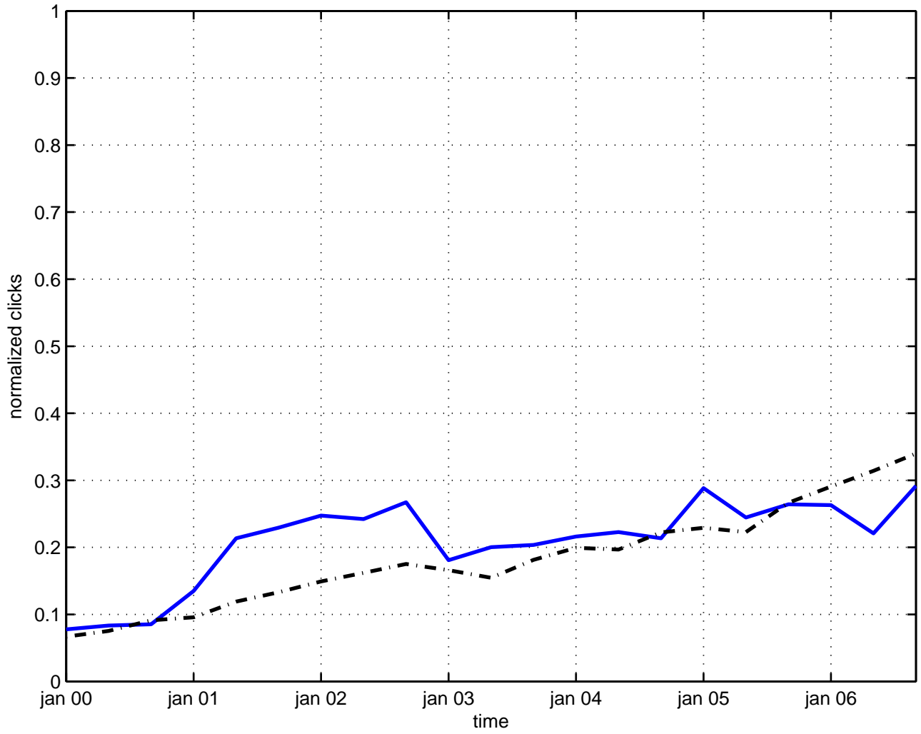
gauge field theory
