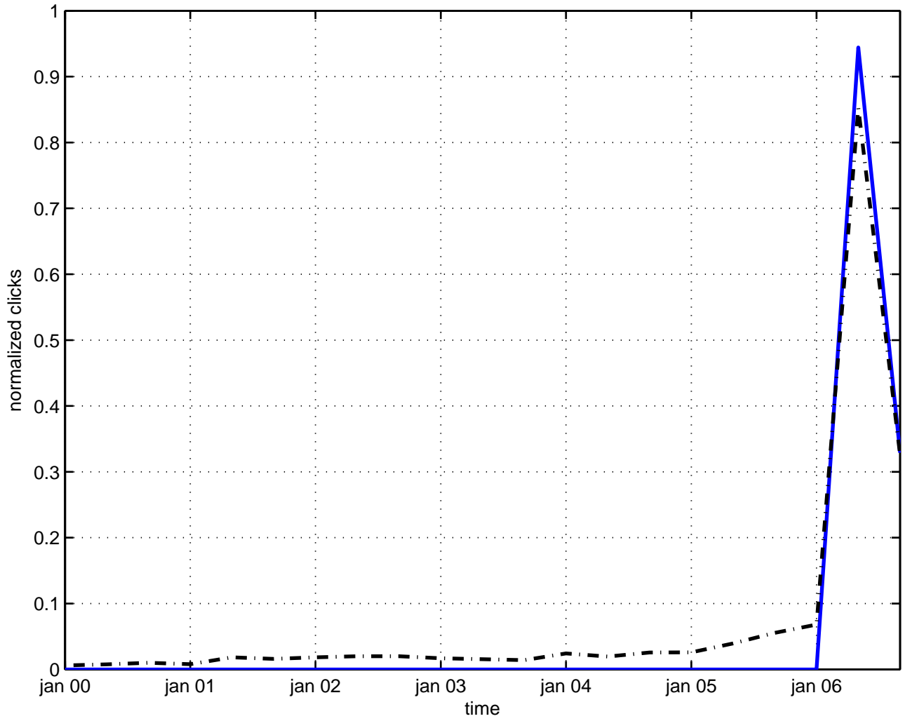
gauge covariance
