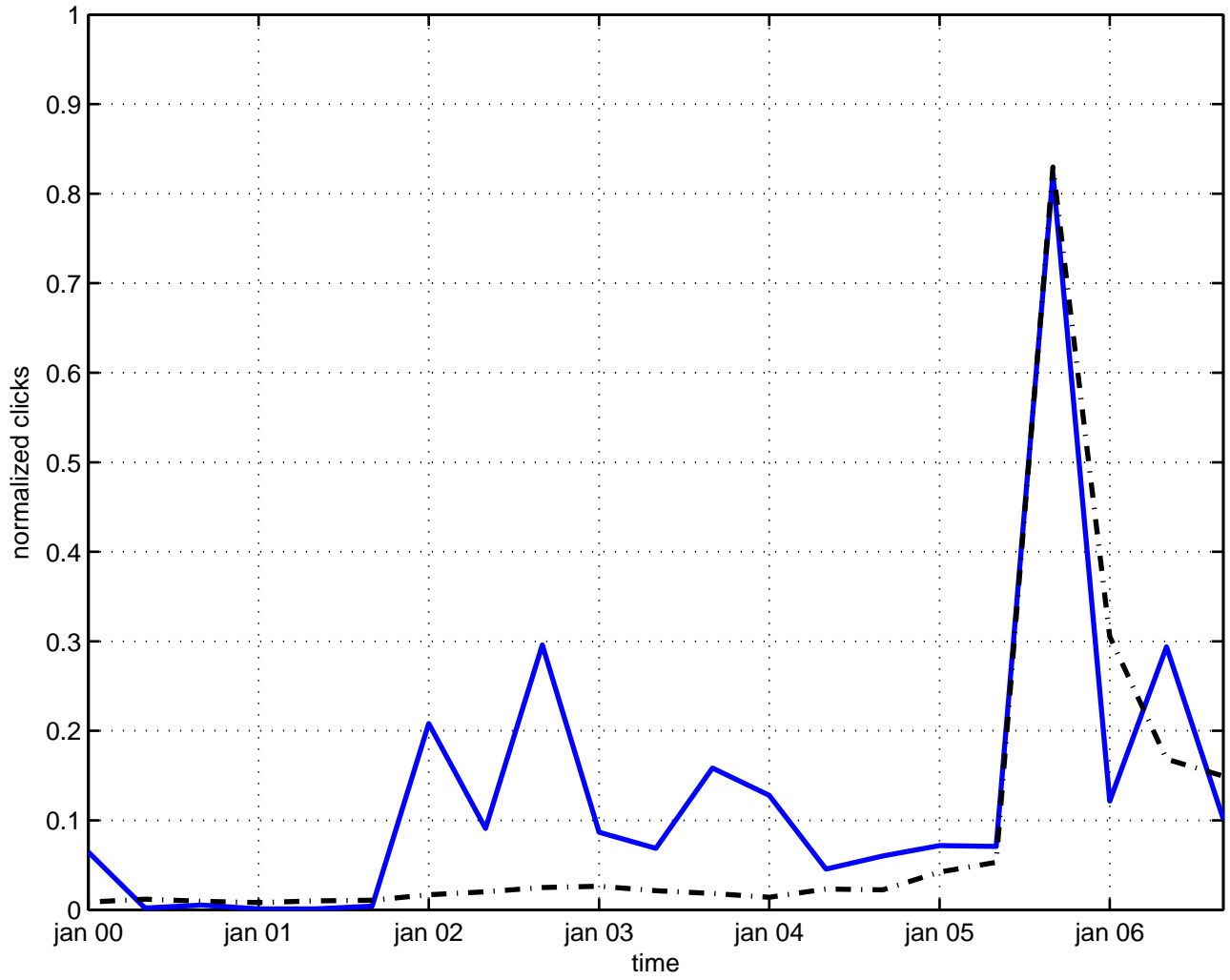
gauge coupling constant
