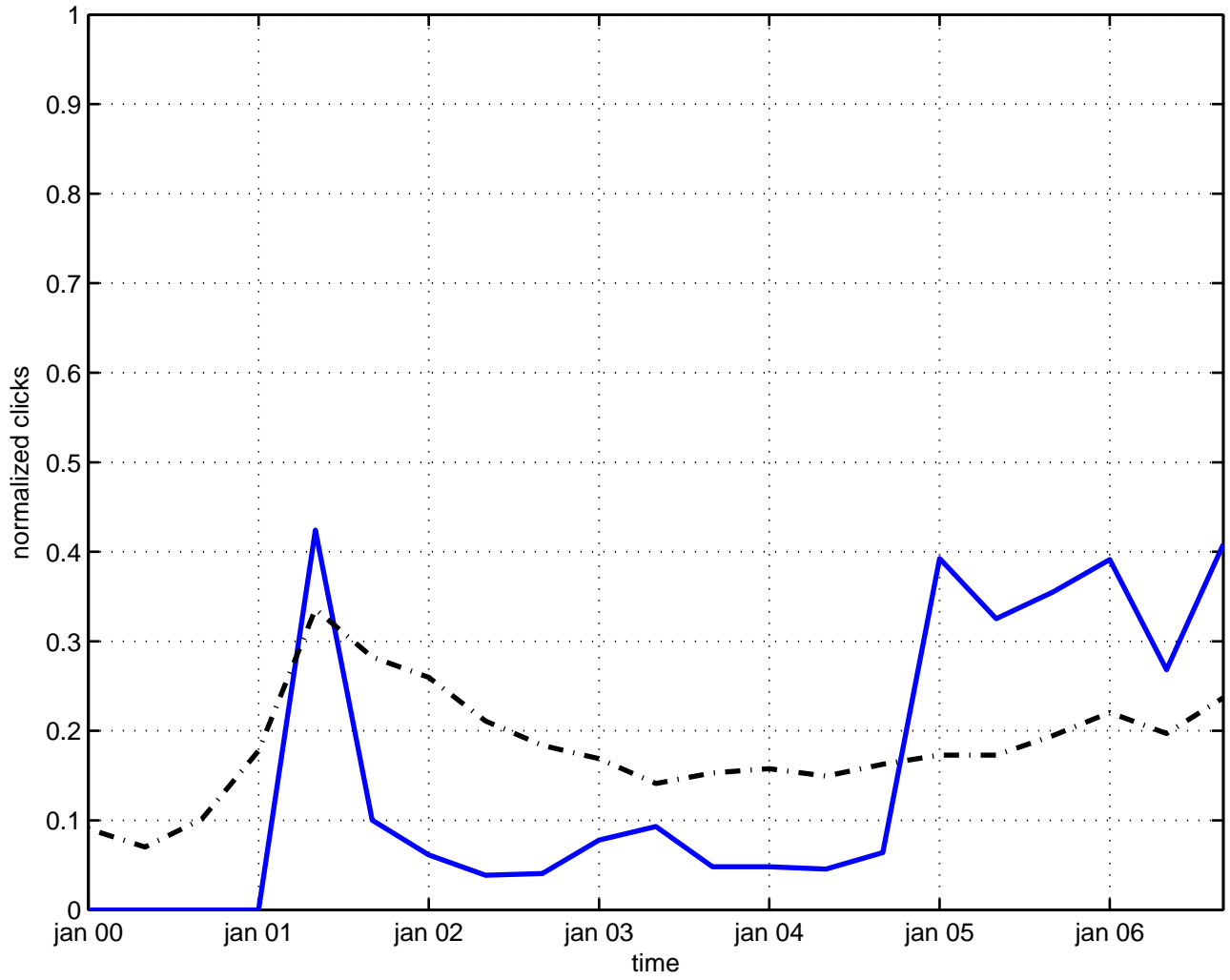
gauge algebra
