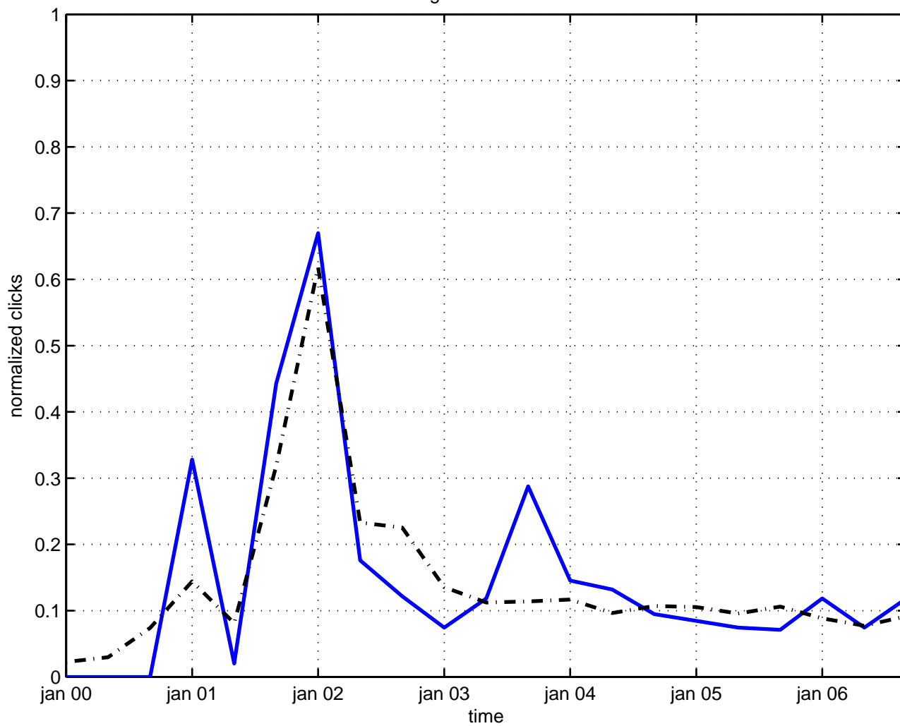
gaudin model
