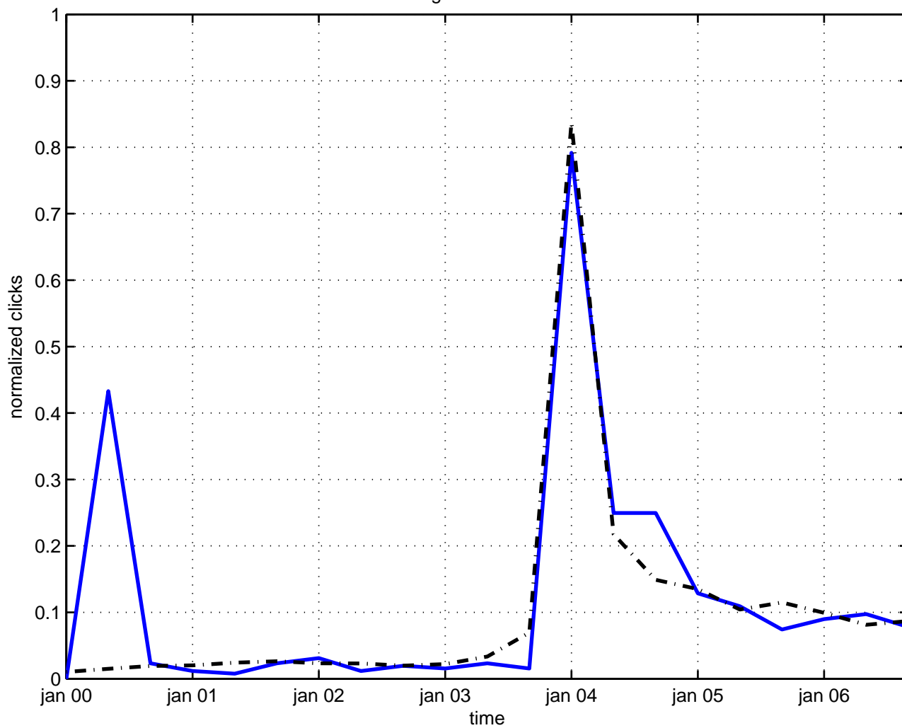
gas instanton
