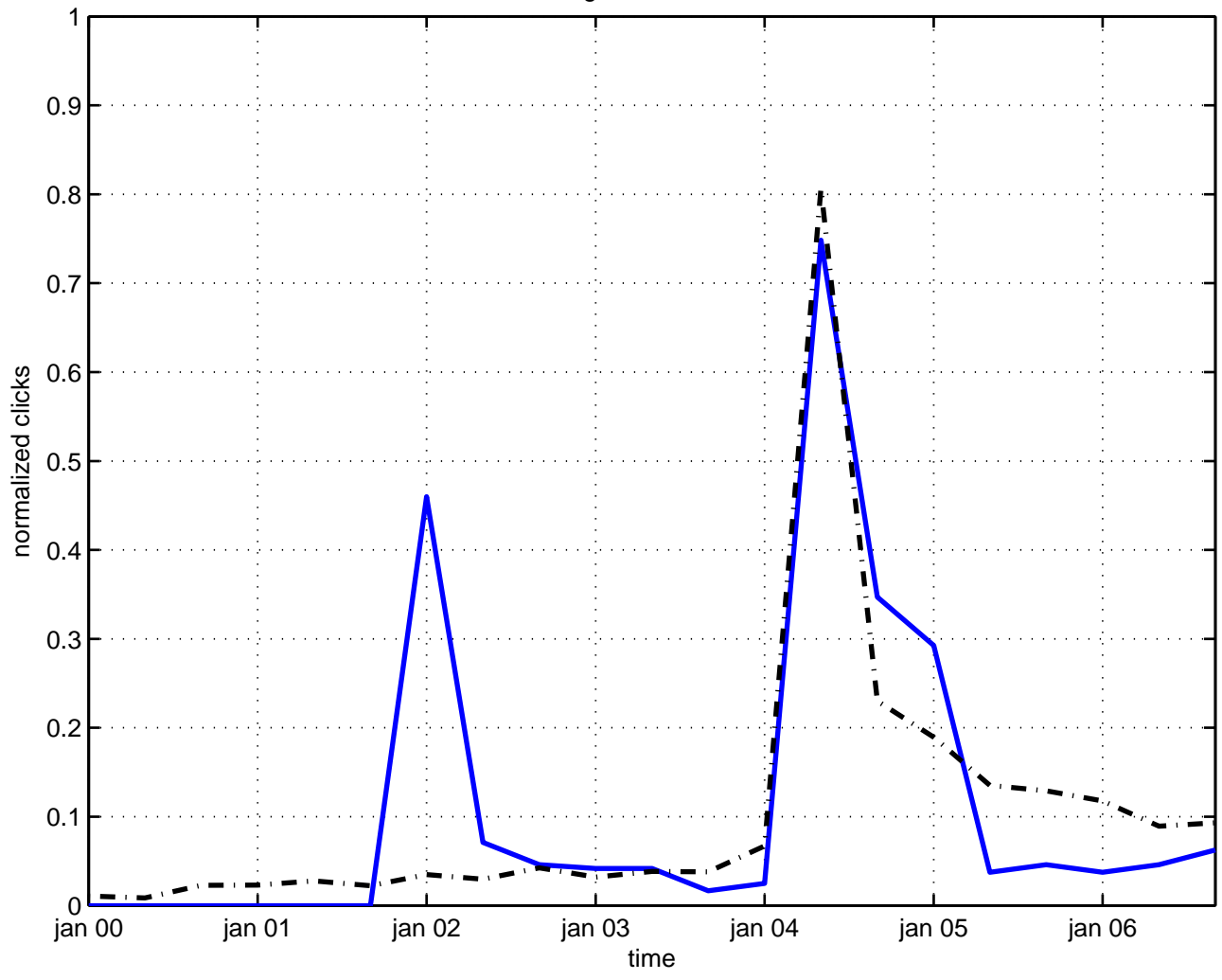
gas electron
