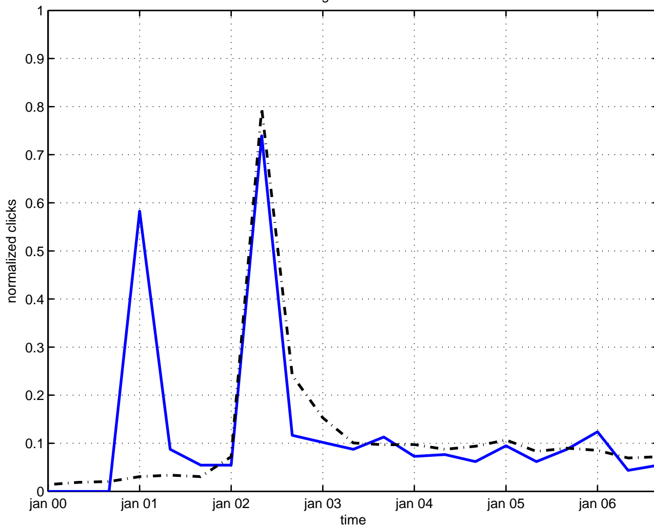
gas boson
