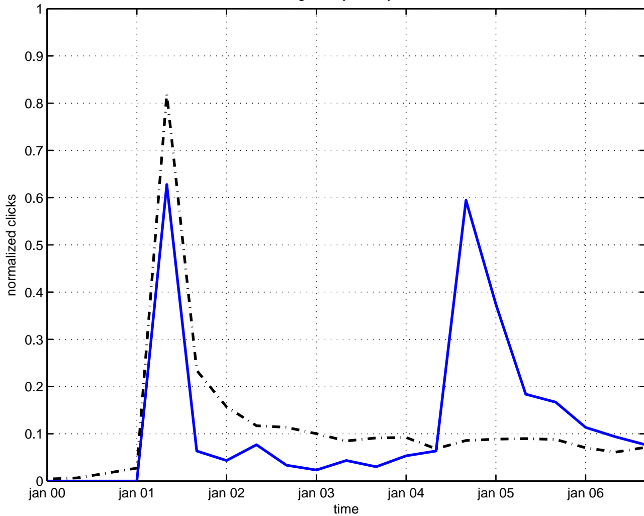
galilei symmetry
