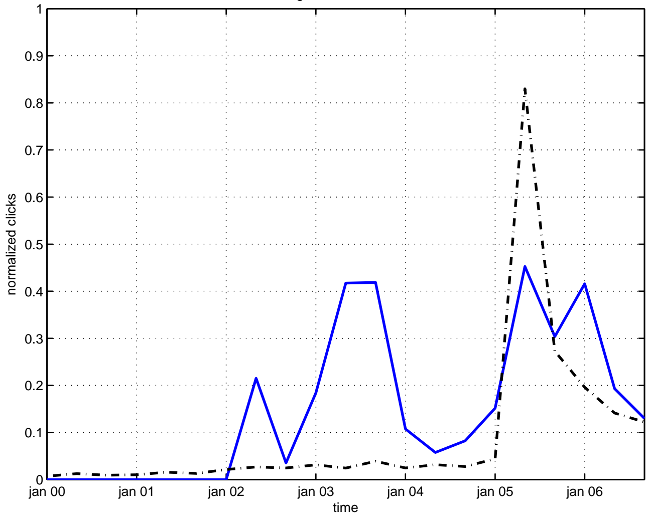
galilei invariance
