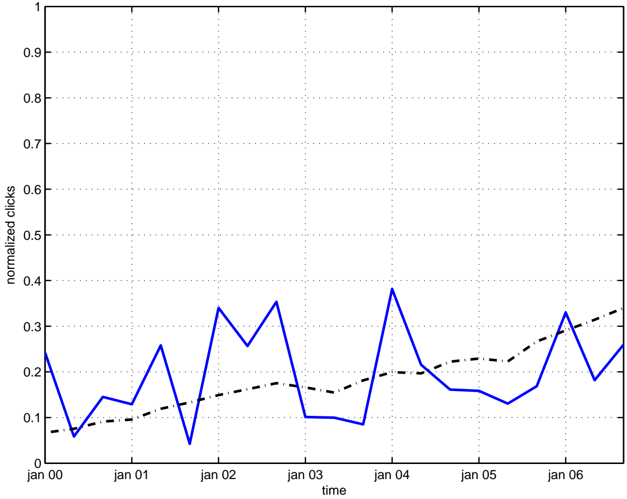
galilei group theory
