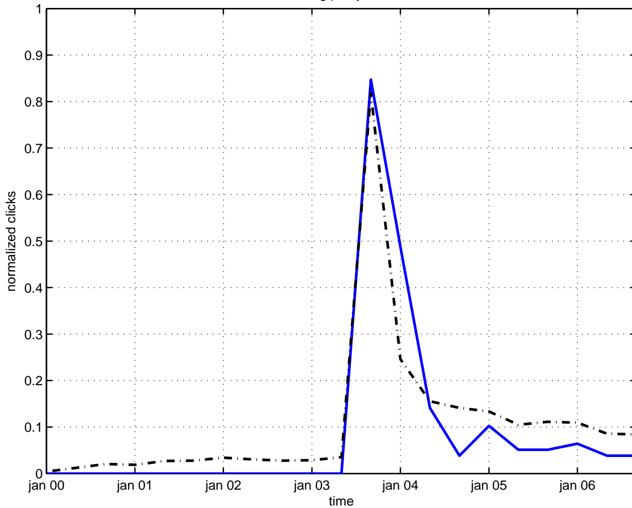
g parity
