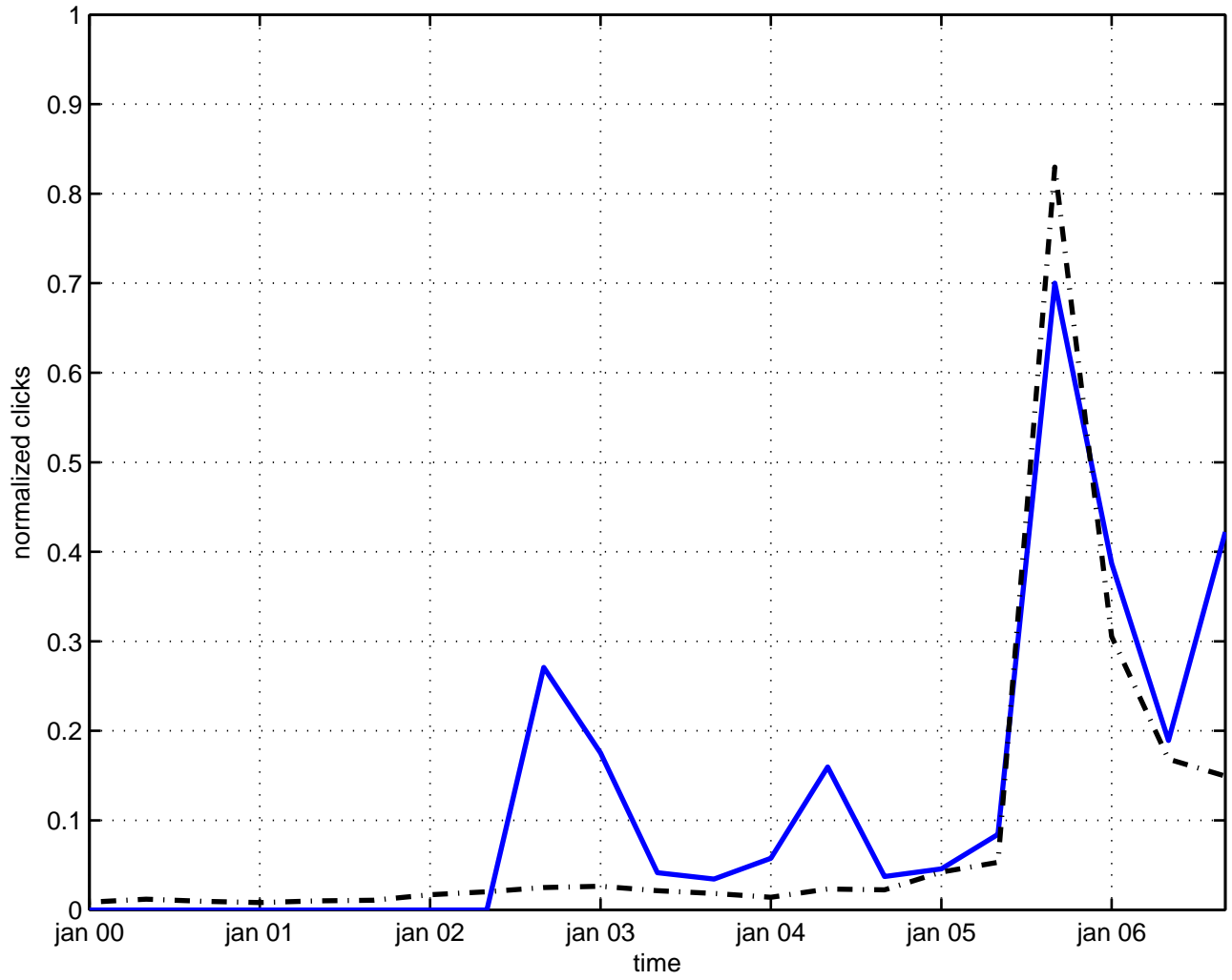
g(2) symmetry
