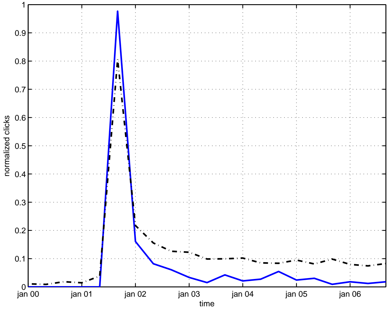
g(2) spontaneous compactification
