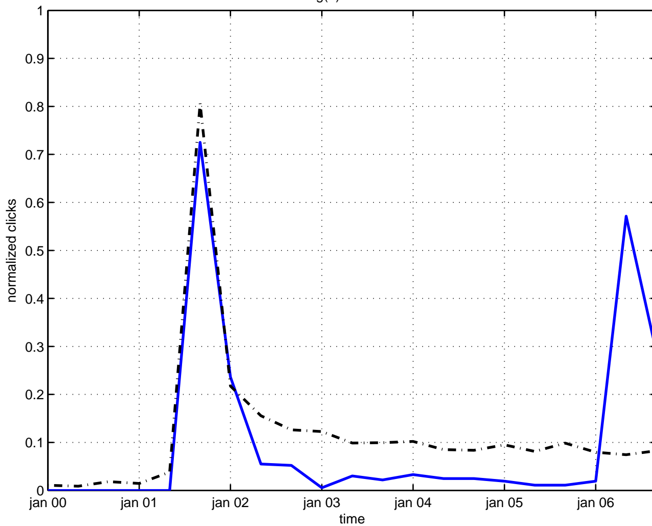
g(2) orbifold
