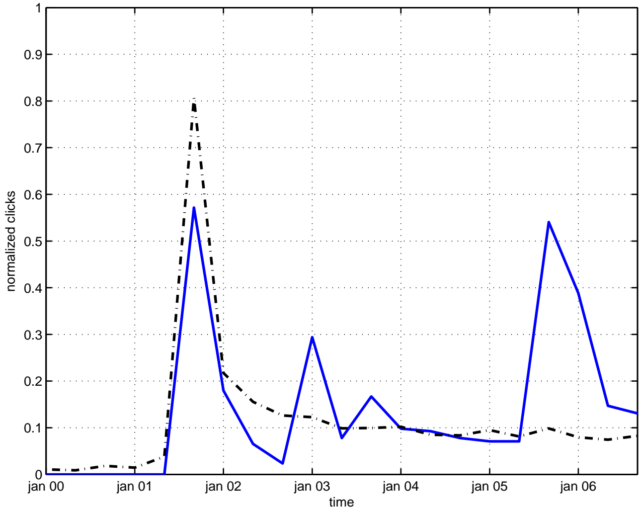
g(2) invariance
