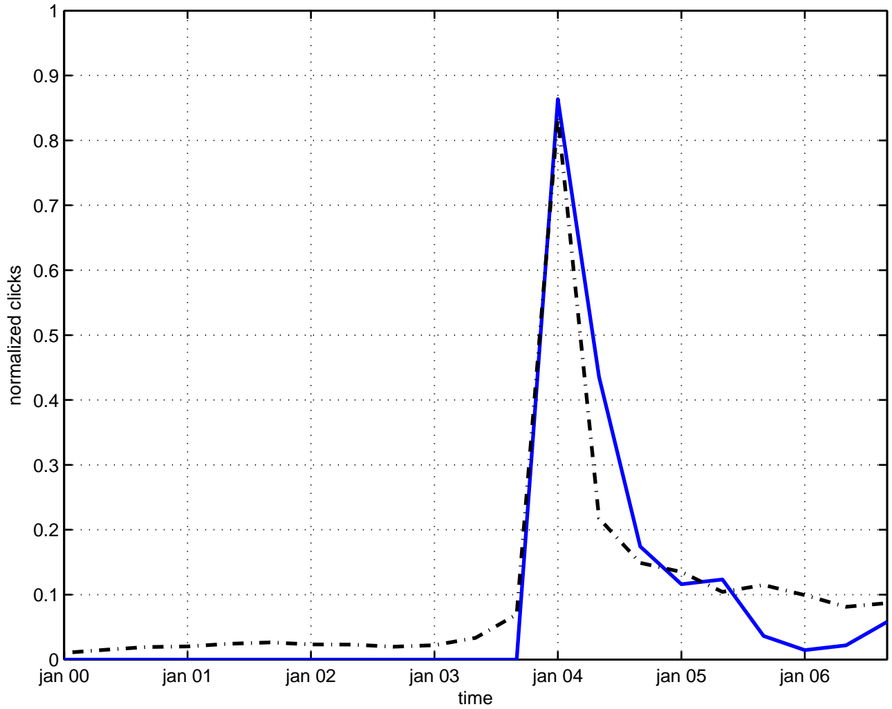
g(11) group theory
