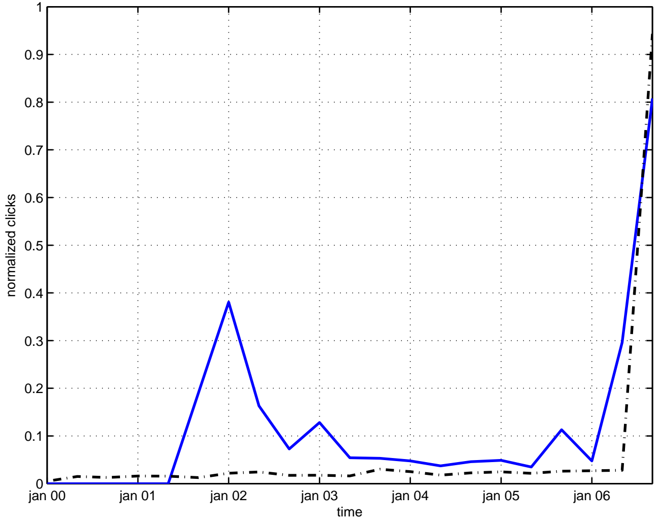
fuzzy space-time
