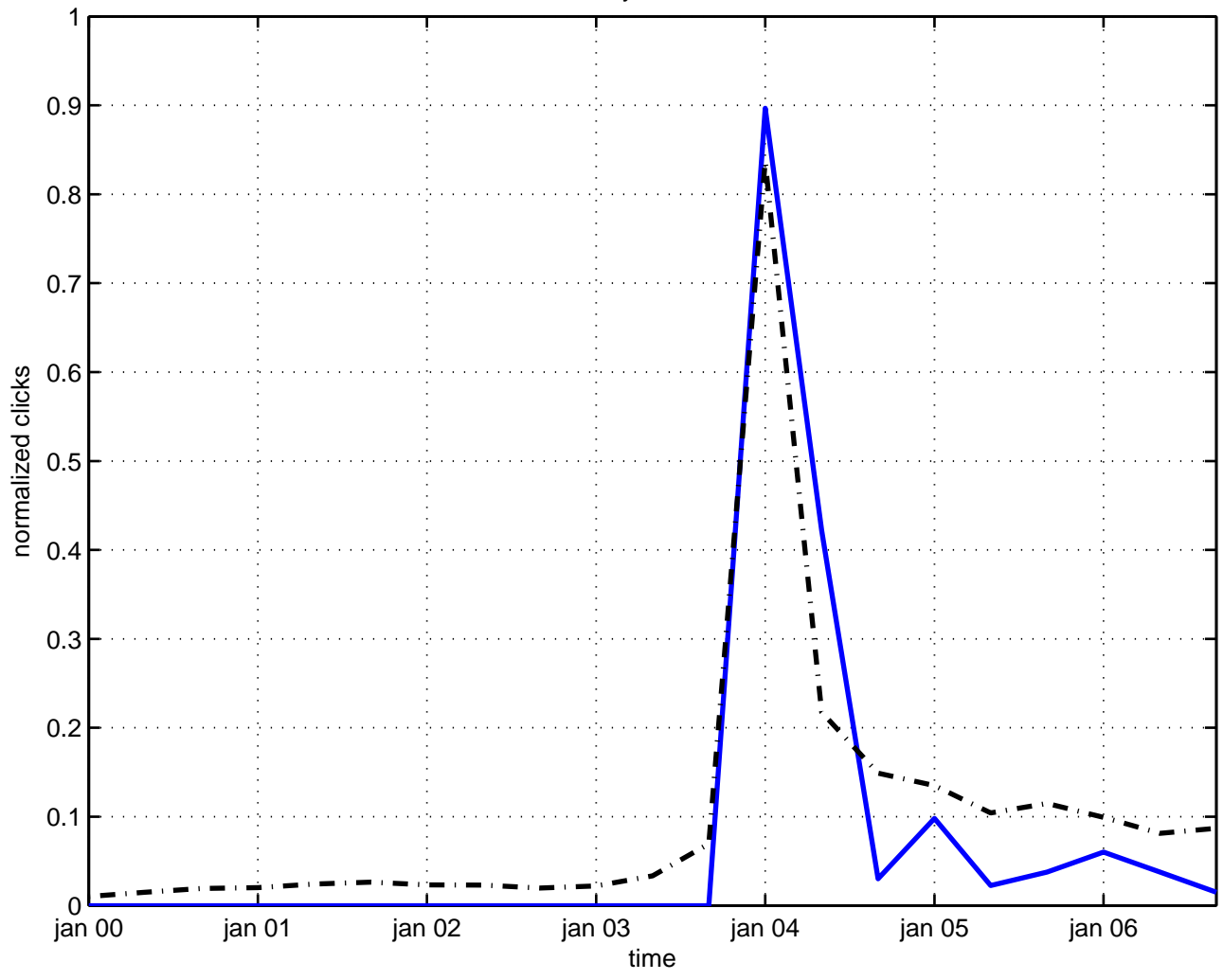
fuzzy solution
