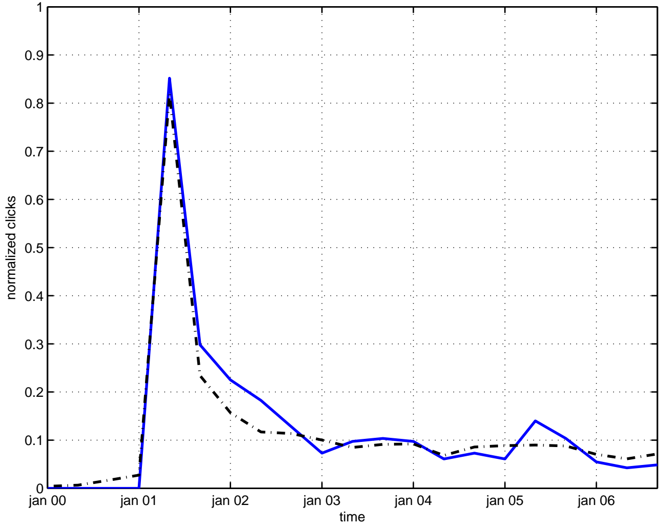
fuzzy instanton
