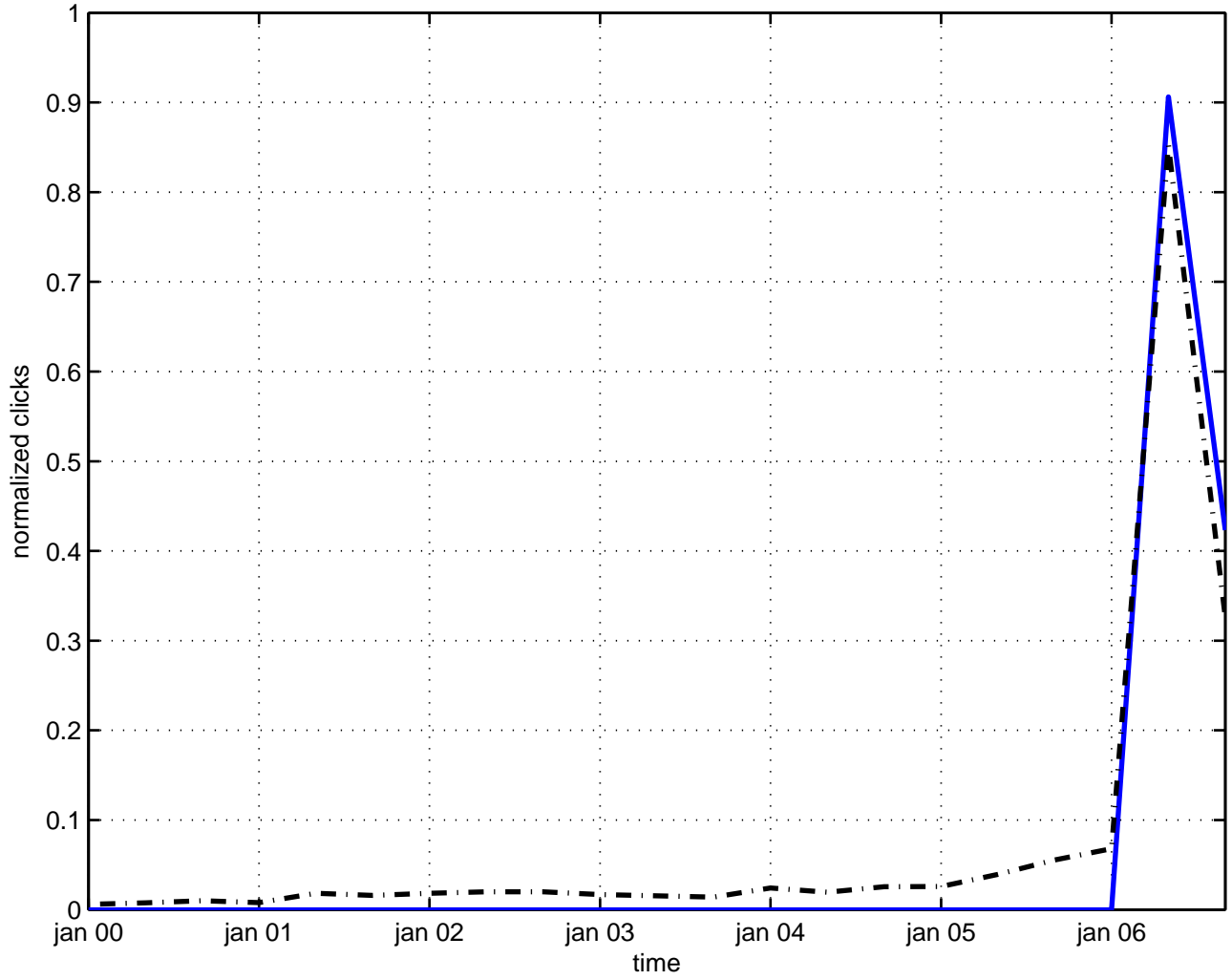
fuzzy horizon
