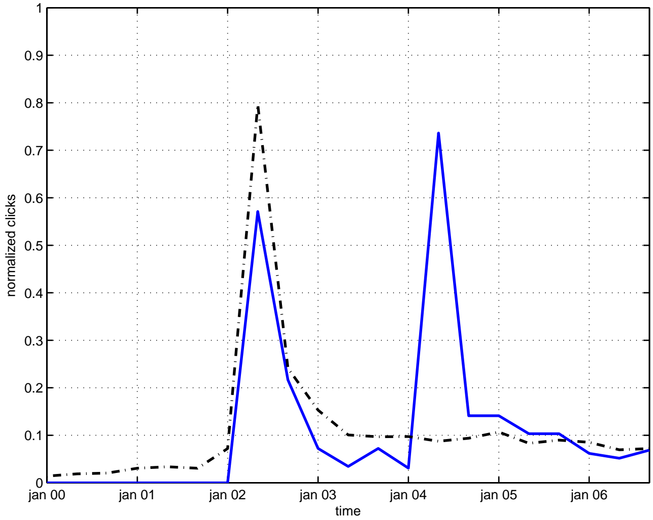
fuzzy geometry
