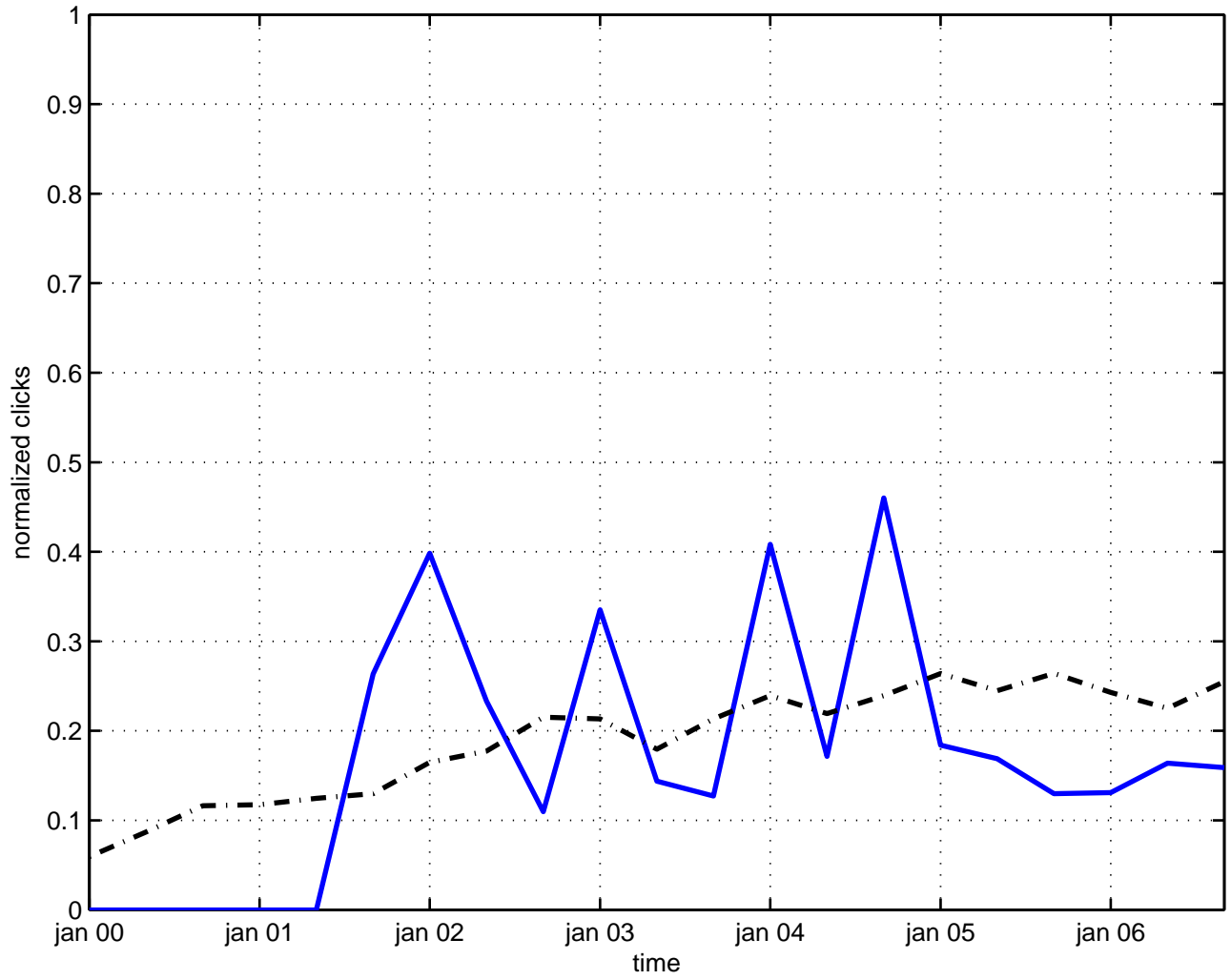
frobenius algebra
