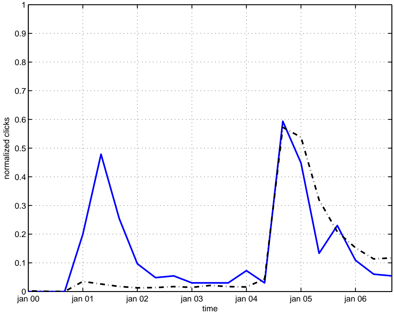
freedman-townsend model
