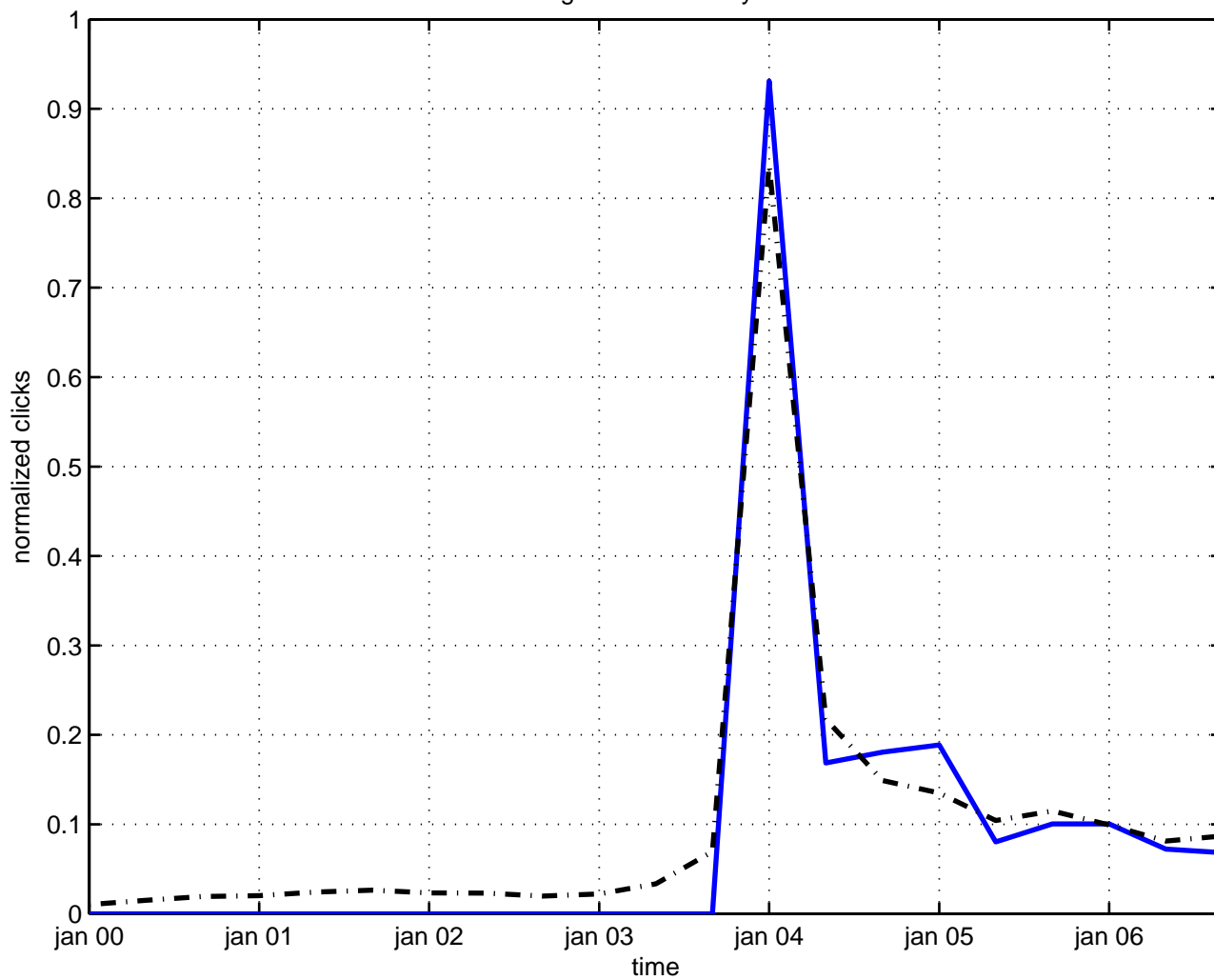
fragmentation tachyon
