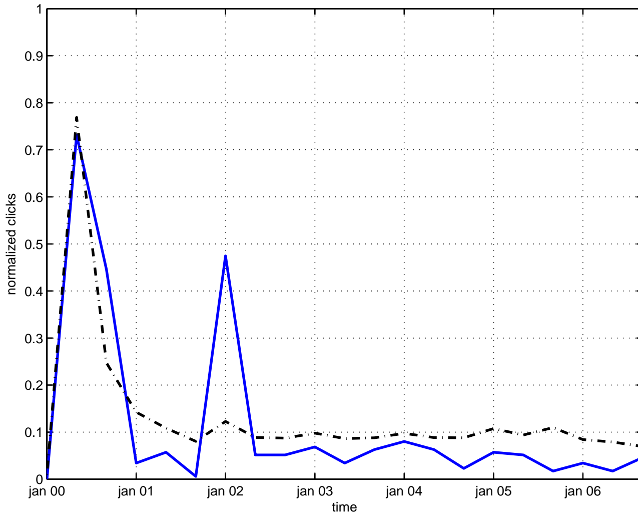
fracton
