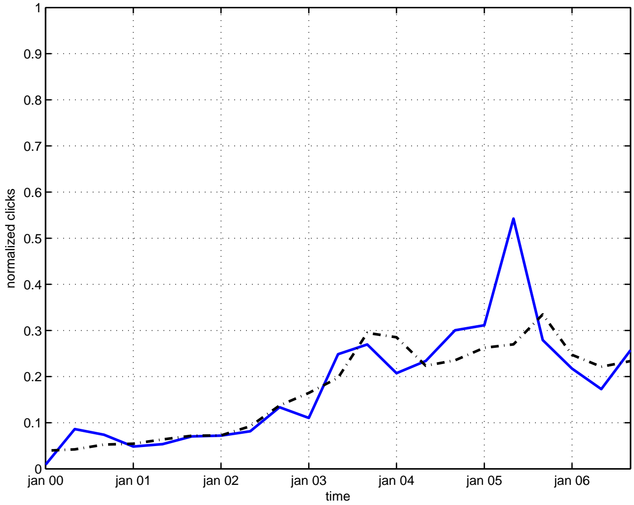
fractional supersymmetry
