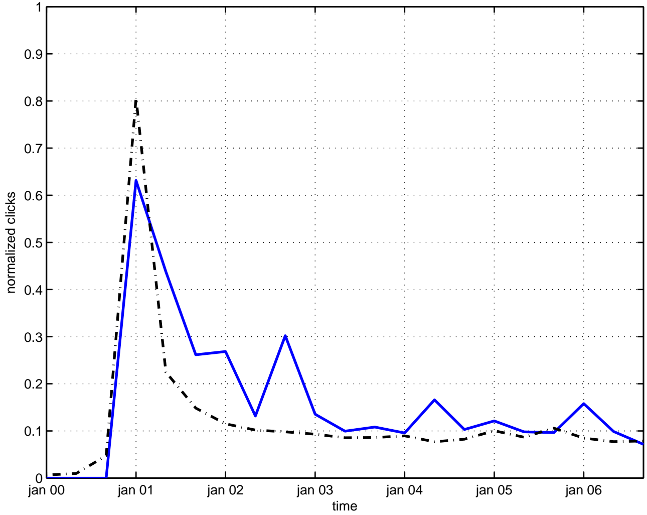
fractional statistics
