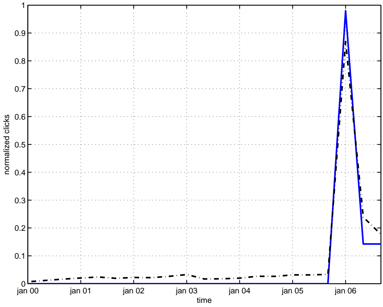
fractional s-brane
