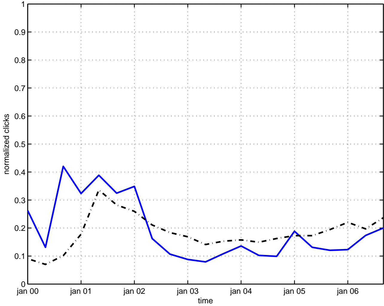
fractional membrane model
