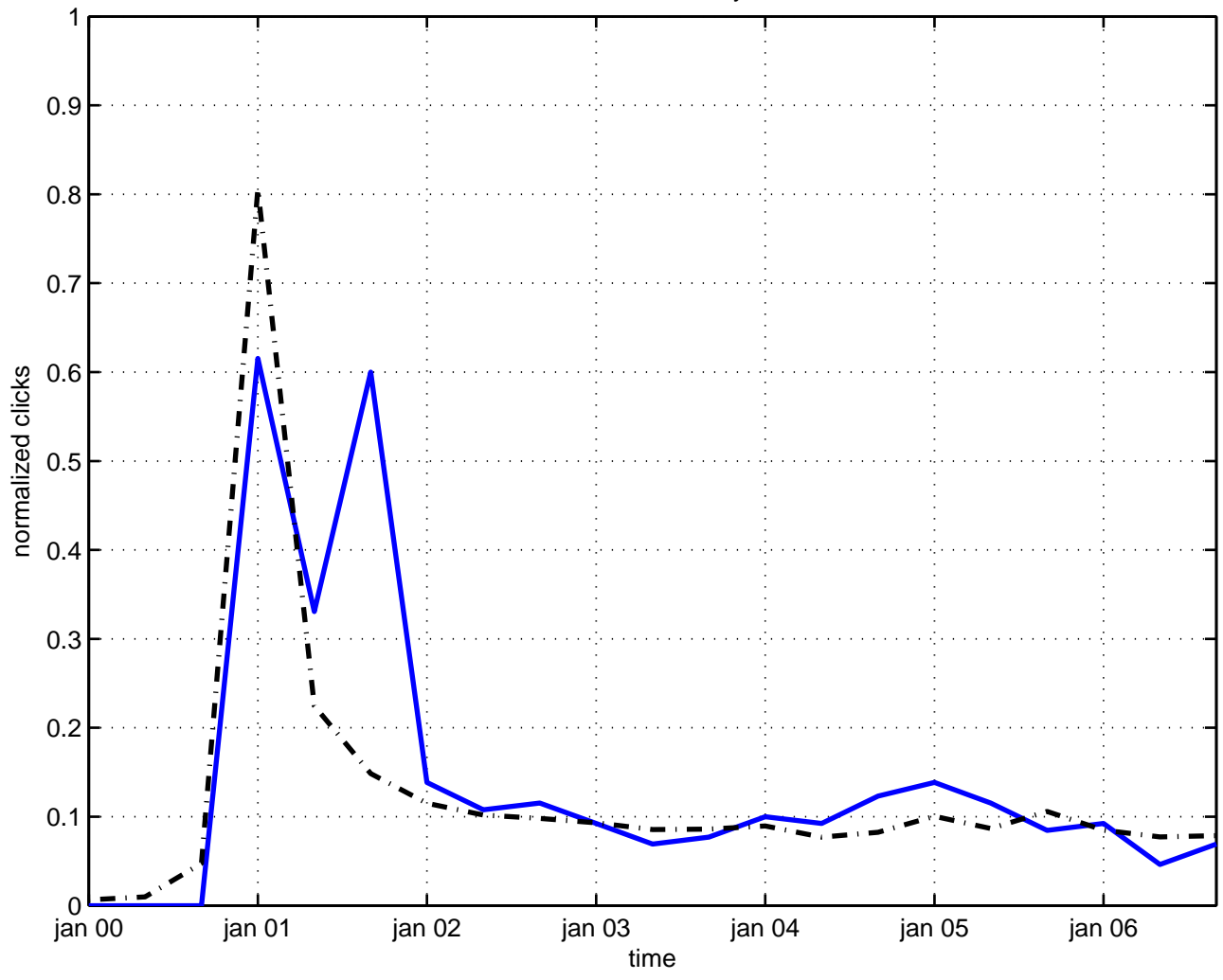
fractional helicity
