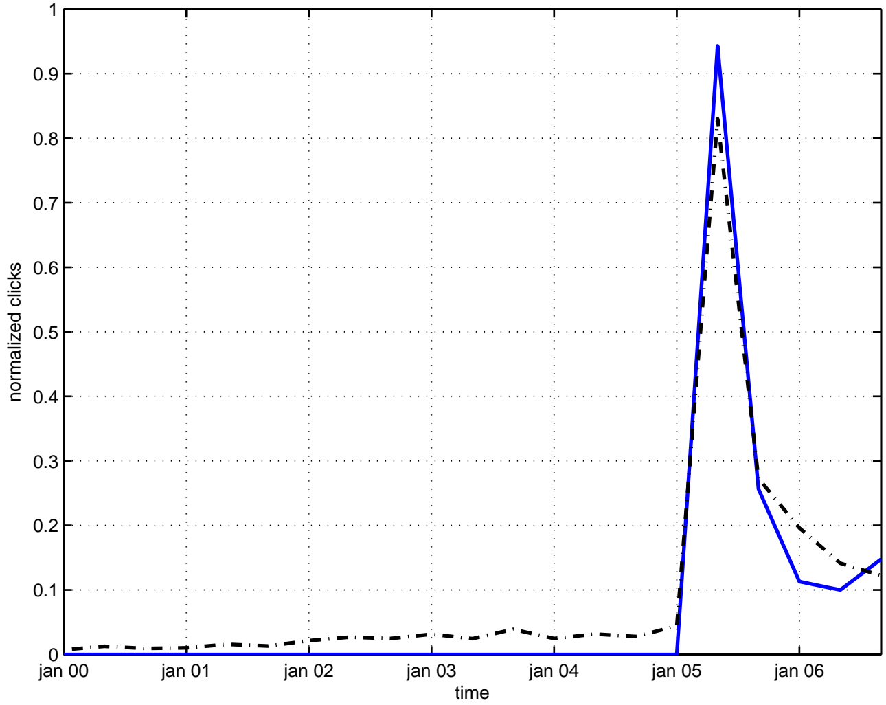
fractional domain wall
