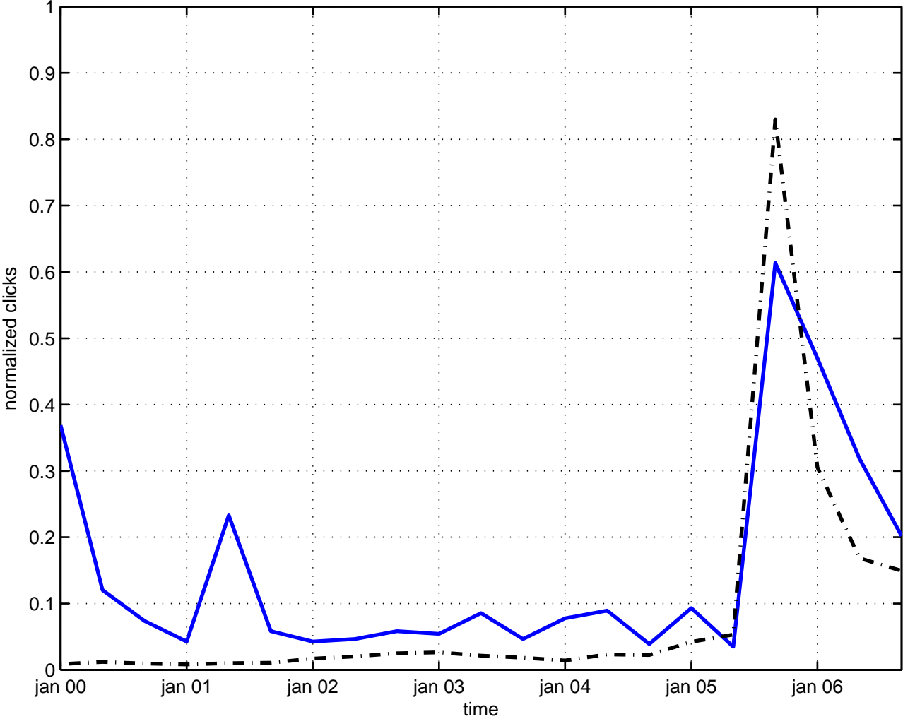
fractional derivative
