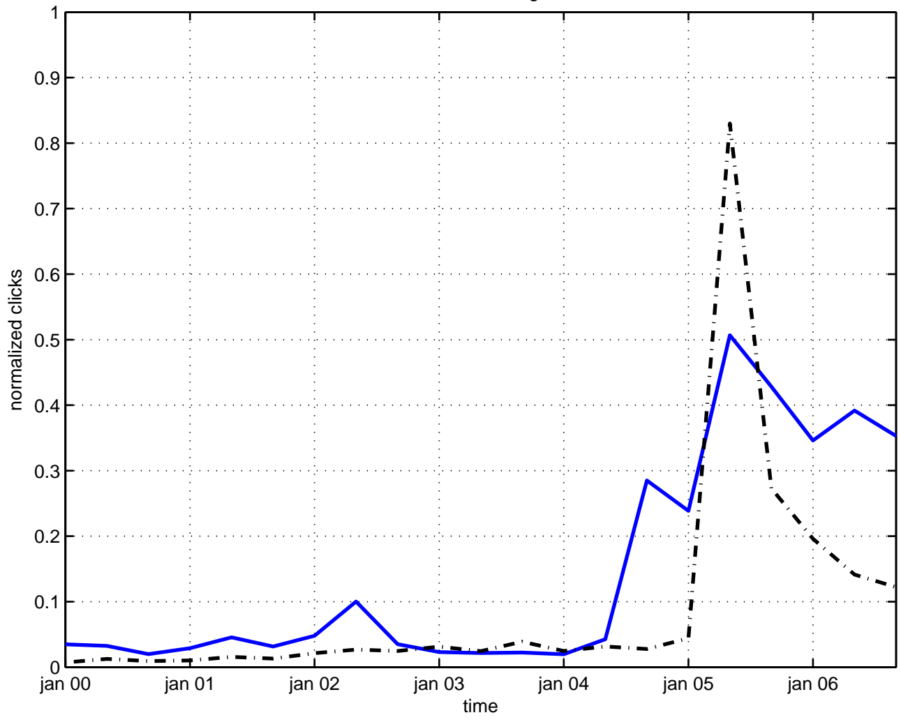
fractional charge
