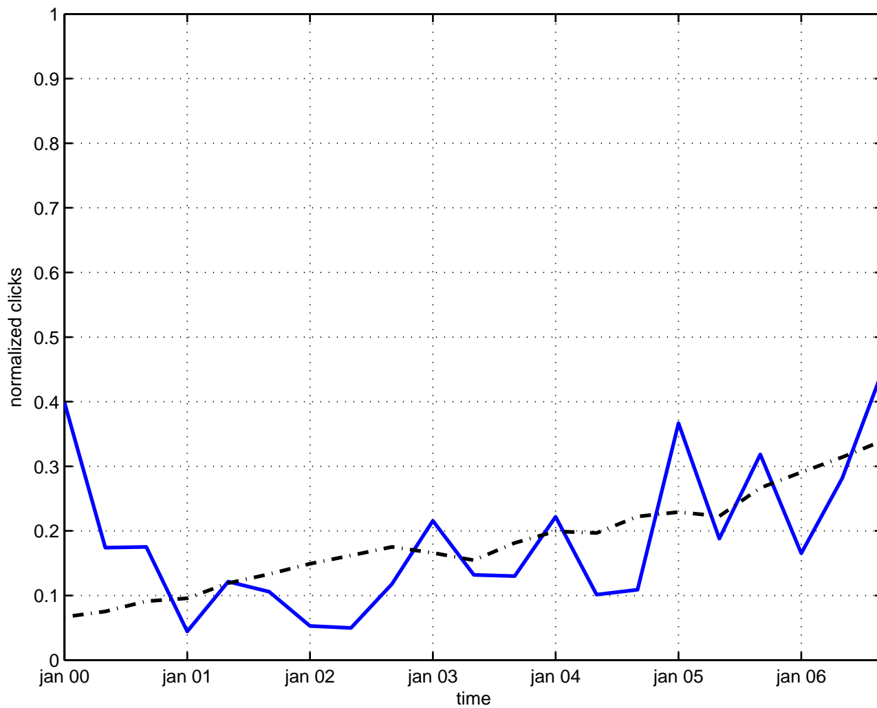
fractal
