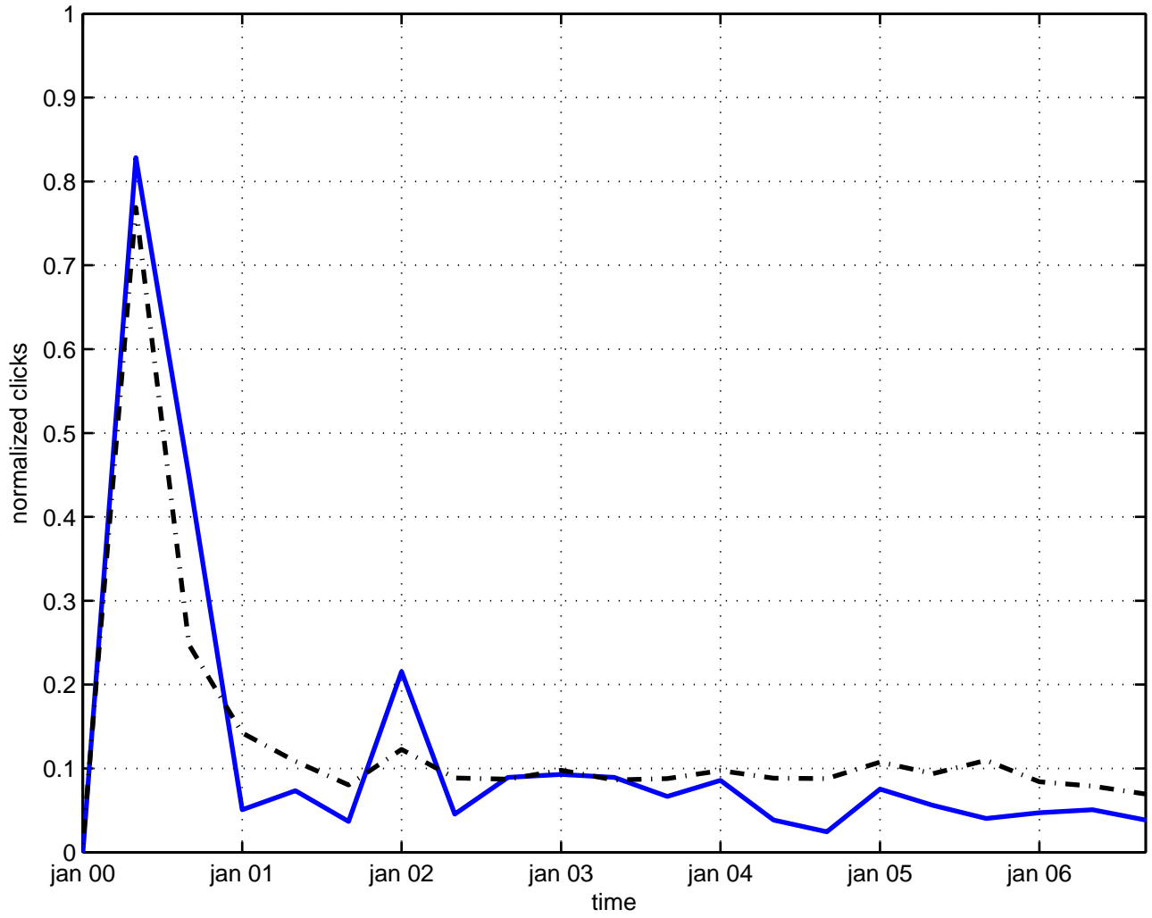
fractal statistics
