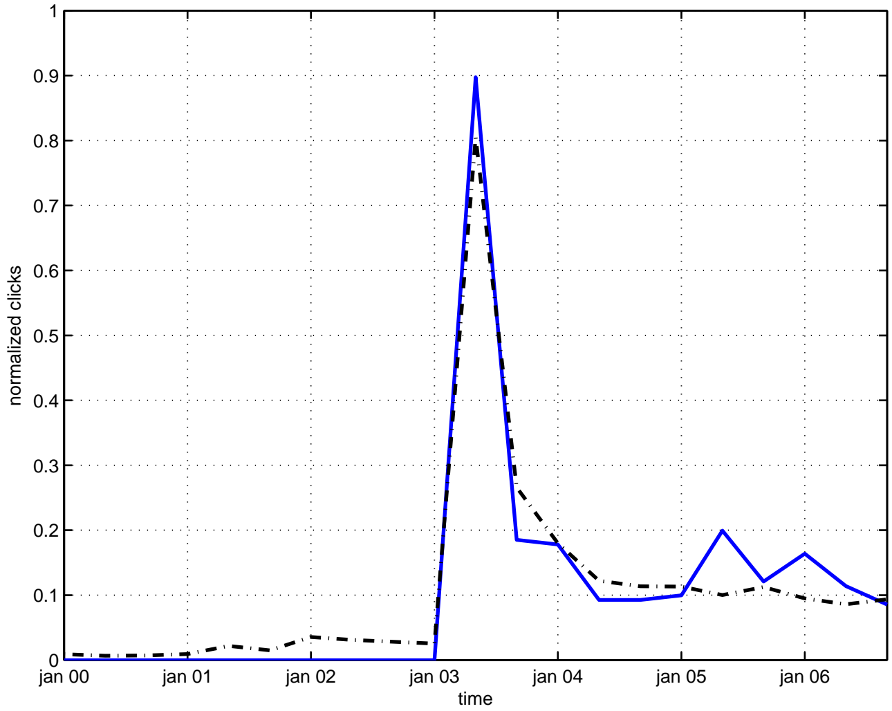
fourier expansion
