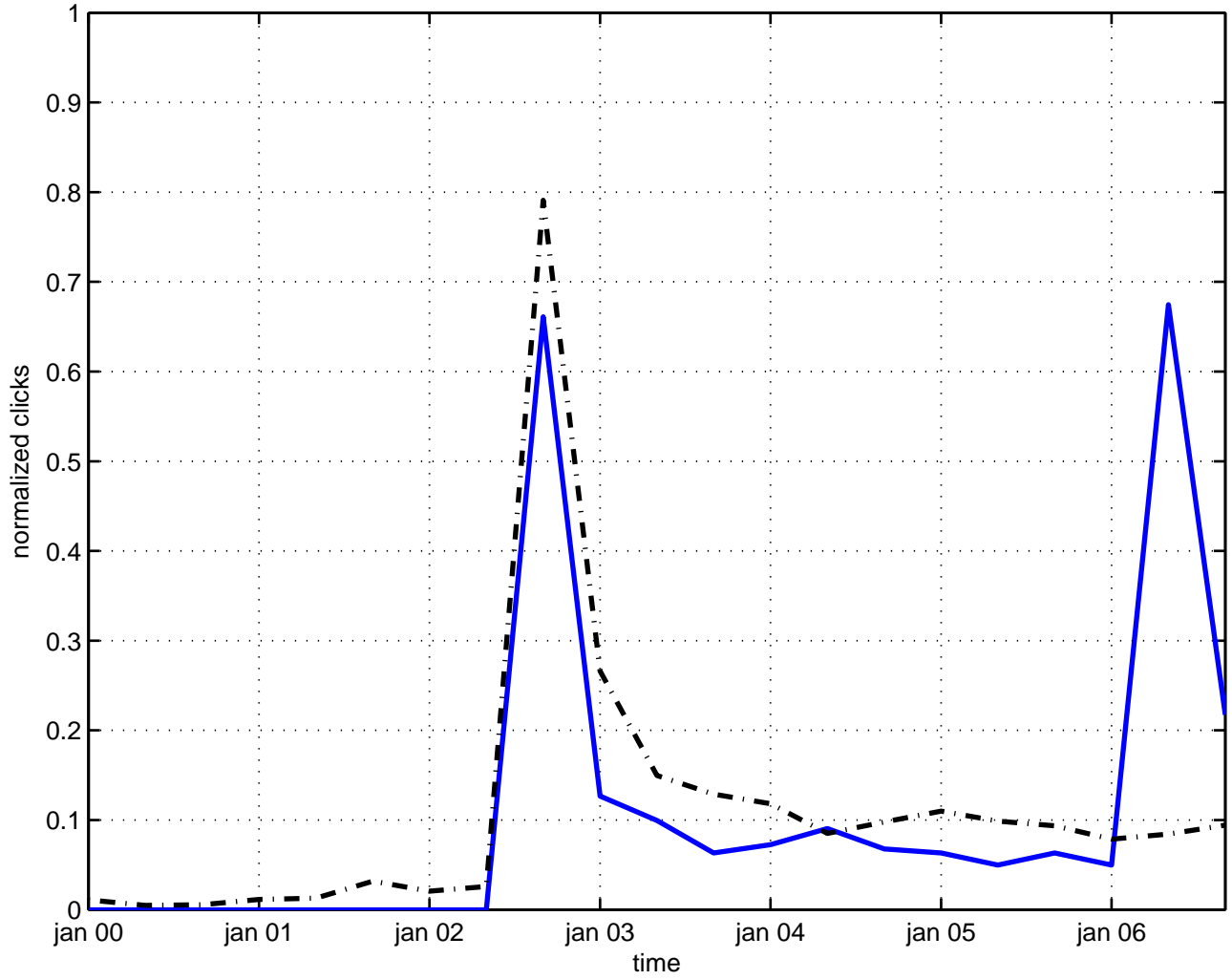
forward scattering
