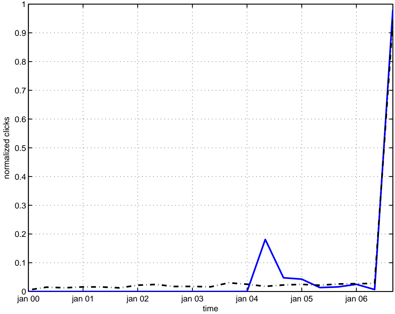
formation horizon
