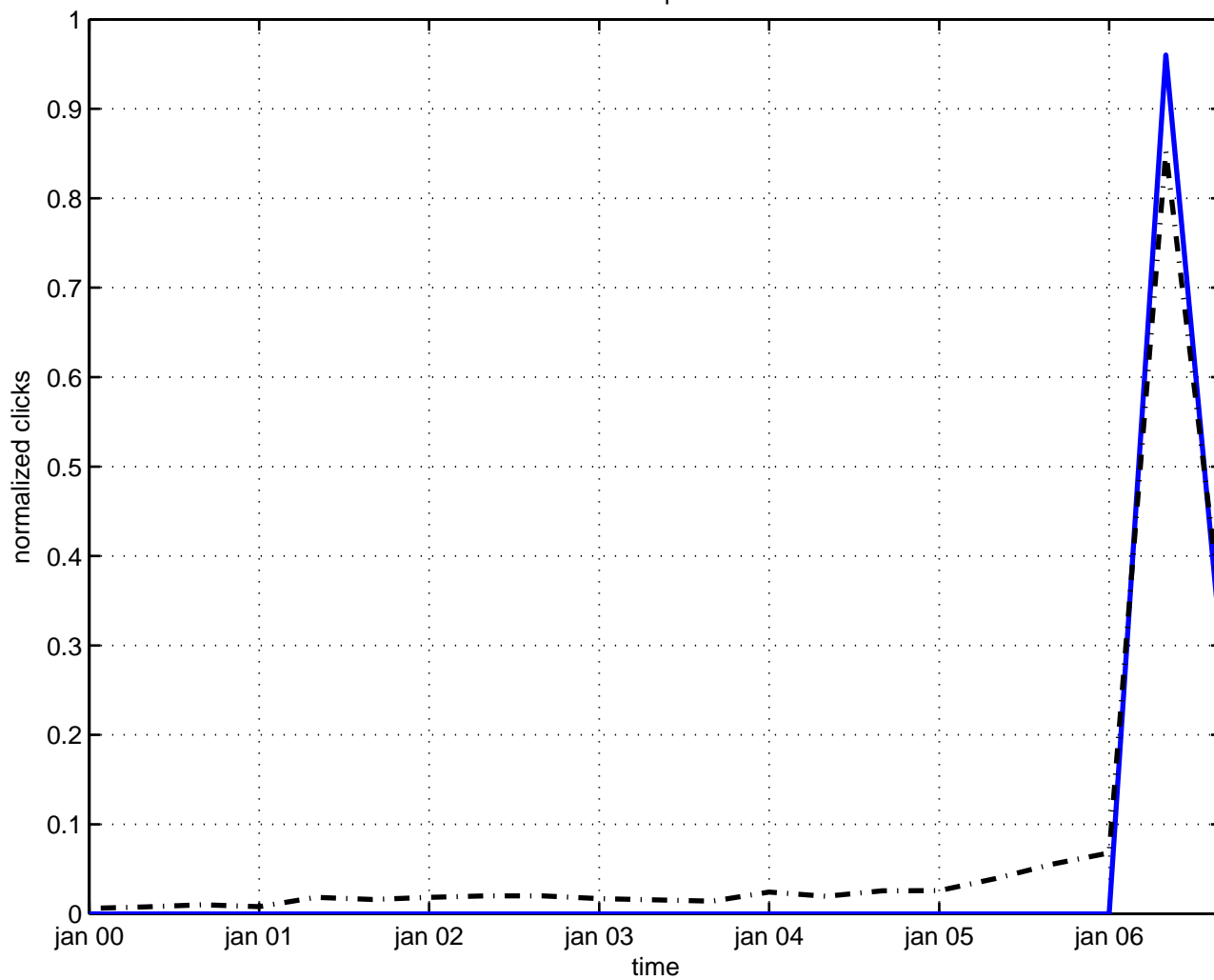
force quark
